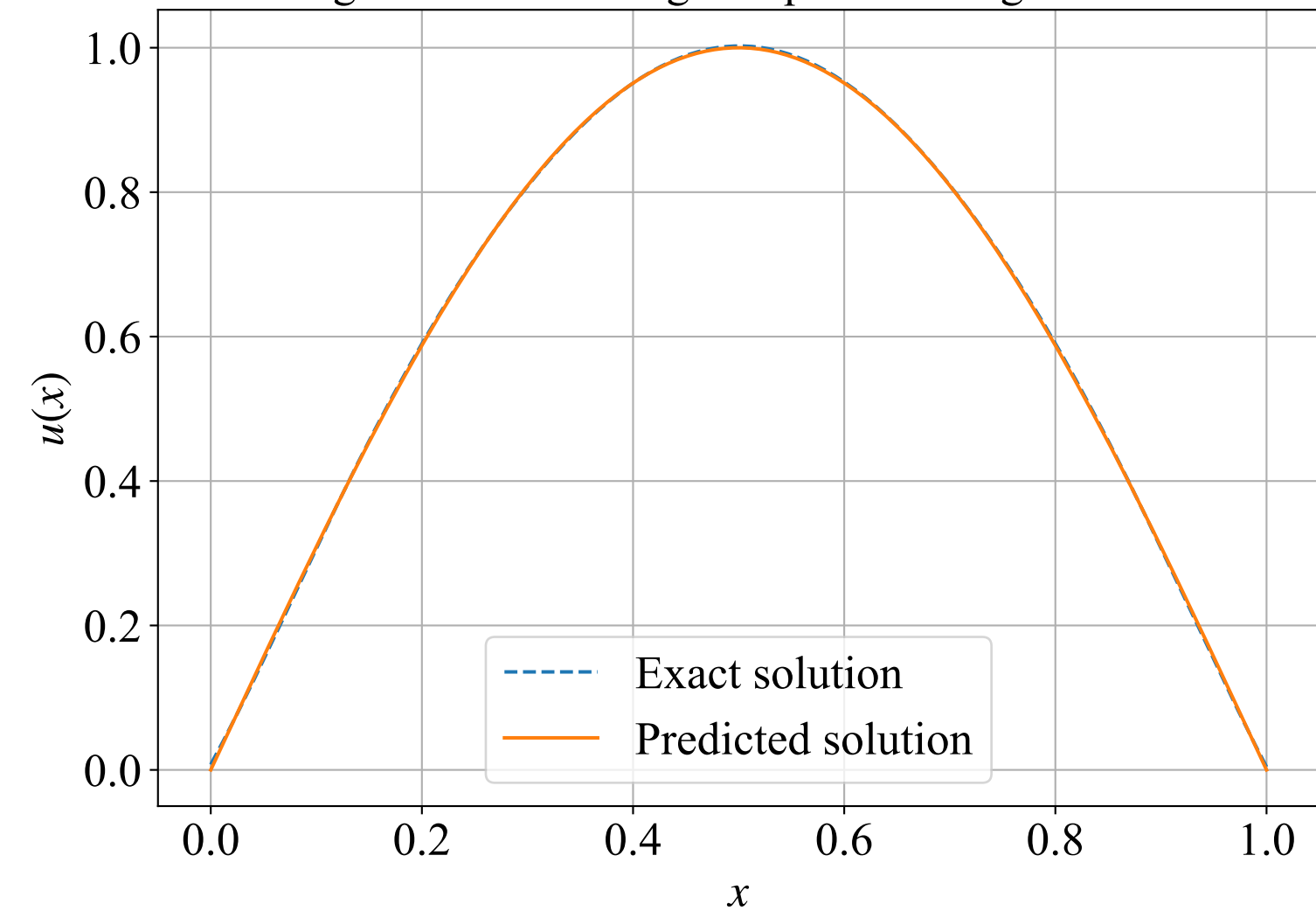
Solving 1D Volterra integral equation using MC-PIKAN
