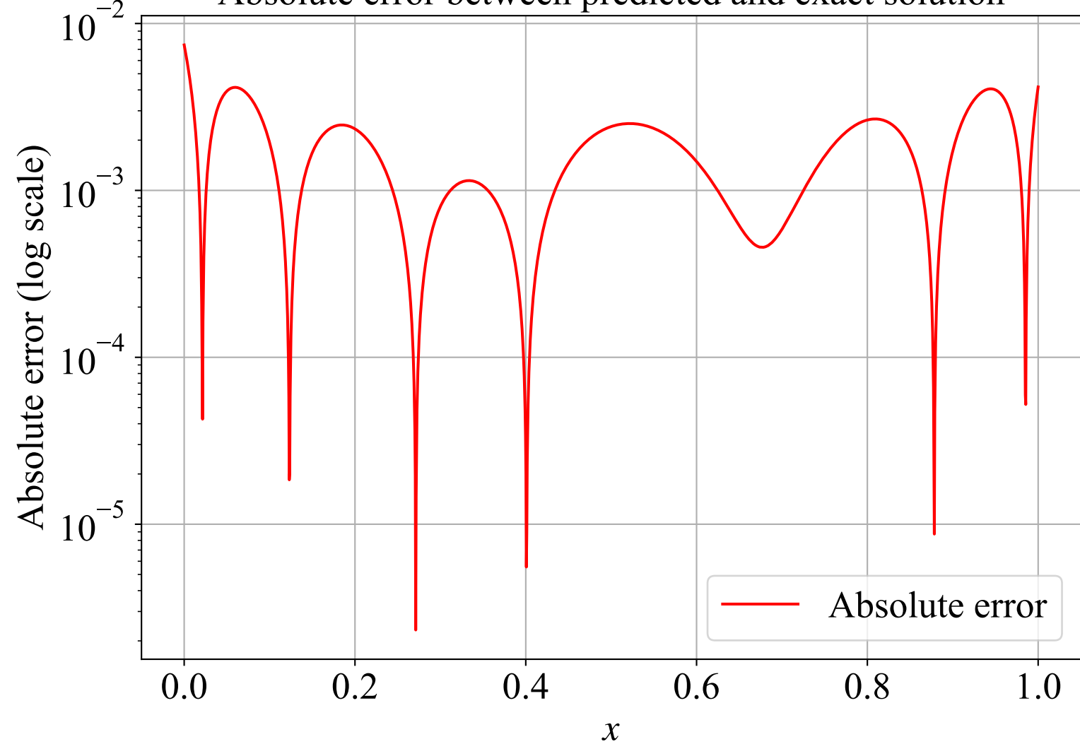
Absolute error between predicted and exact solution
